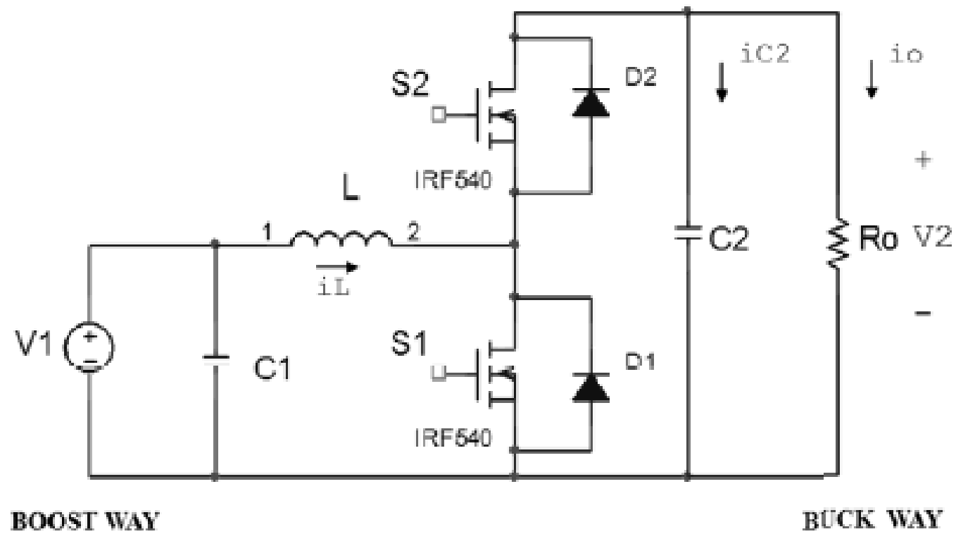
Figure 4. Bidirectional buck-boost DC/DC switching converter
