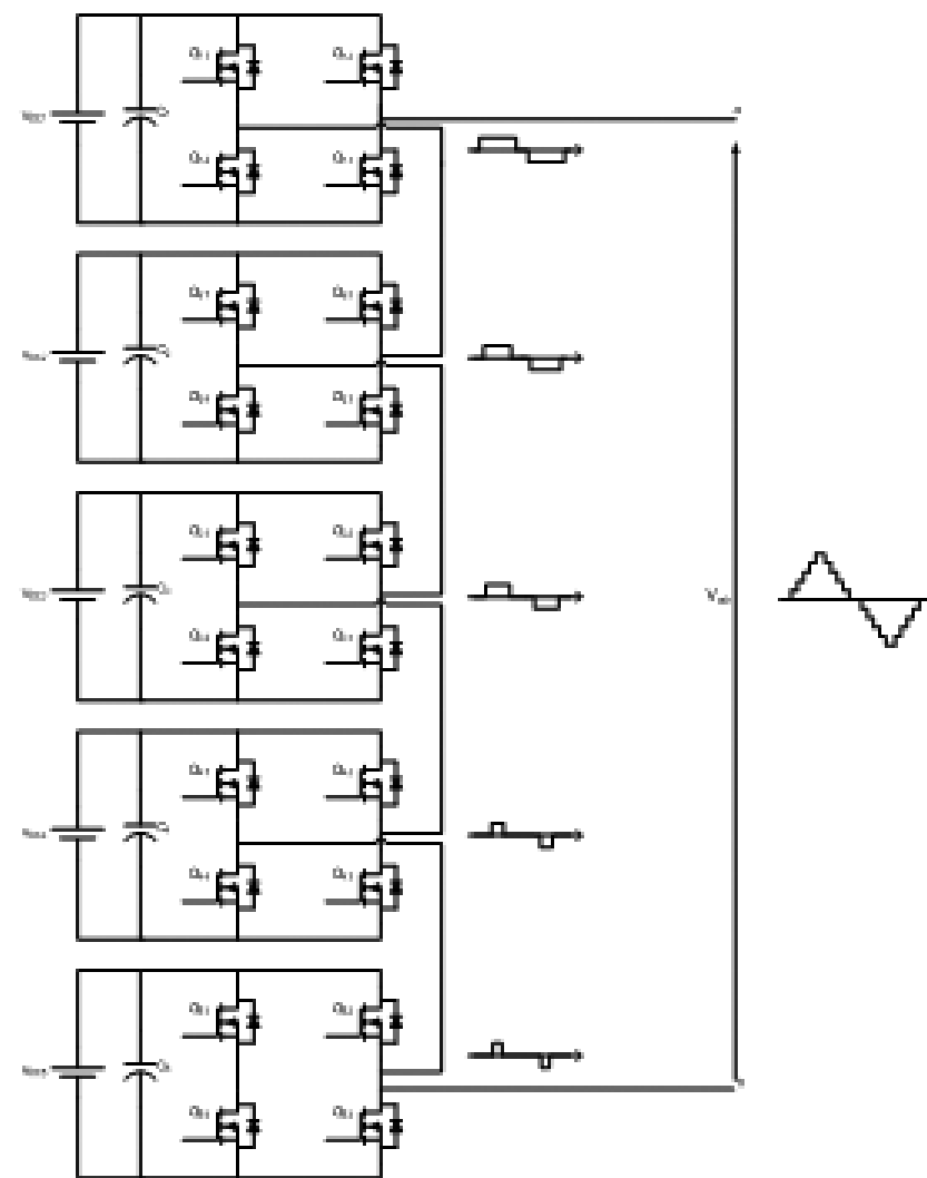
INVERSOR MULTINIVELES
